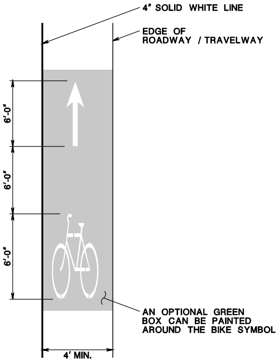
TYPICAL BIKE LANE
