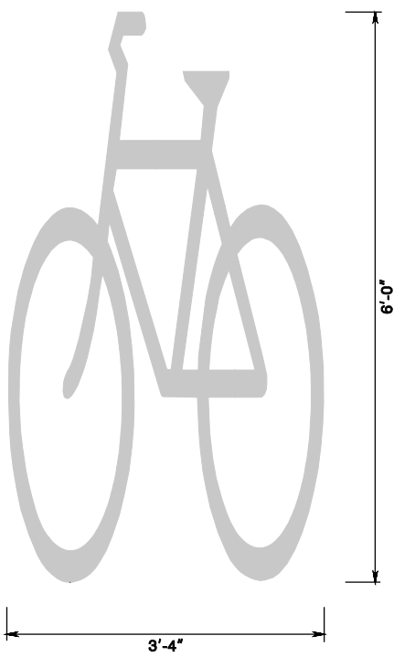
BIKE SYMBOL AREA = 7 S.F.
