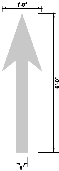
BIKE LANE THROUGH ARROW AREA = 4 S.F.
